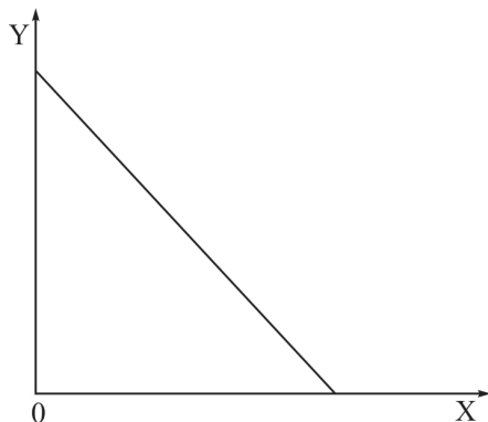
Fig. 3 f'(x) < 0 , f''(x) = 0
