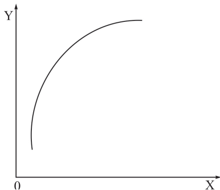
Fig. 5 f'(x) > 0 , f''(x) < 0
